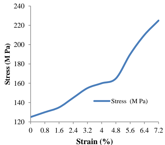
Figure 9: Stress vs Strain (3% Boron)
