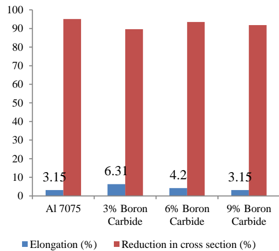
Figure 14: Variation of Elongation and Reduction in Cross Section during Tensile Testing
