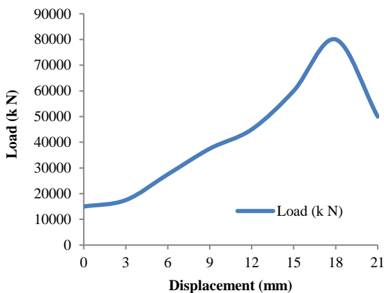
Figure 6: Force vs Displacement (Al 7075)
