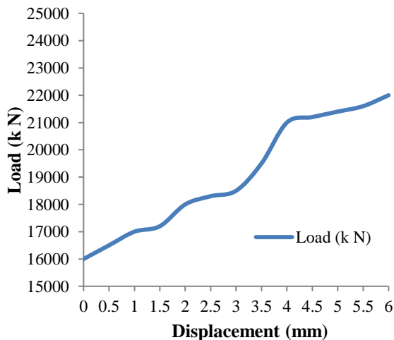
Figure 12: Force vs Displacement (9% Boron)
