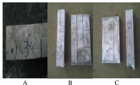
Figure 1: Al- B 4 C Composite Samples (A) 3% B 4 C (B) 6% B 4 C (C) 9% B 4 C
