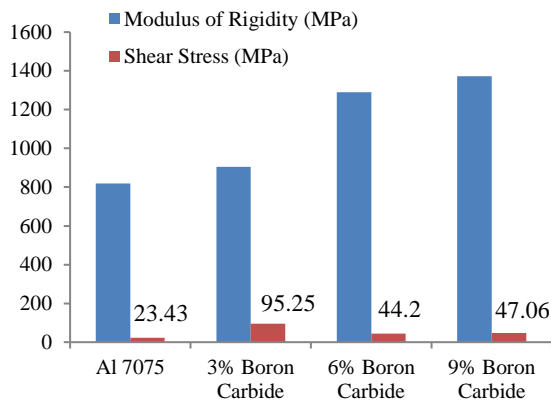
Figure 5: Variation in the Critical Parameters During Tensile Testing
